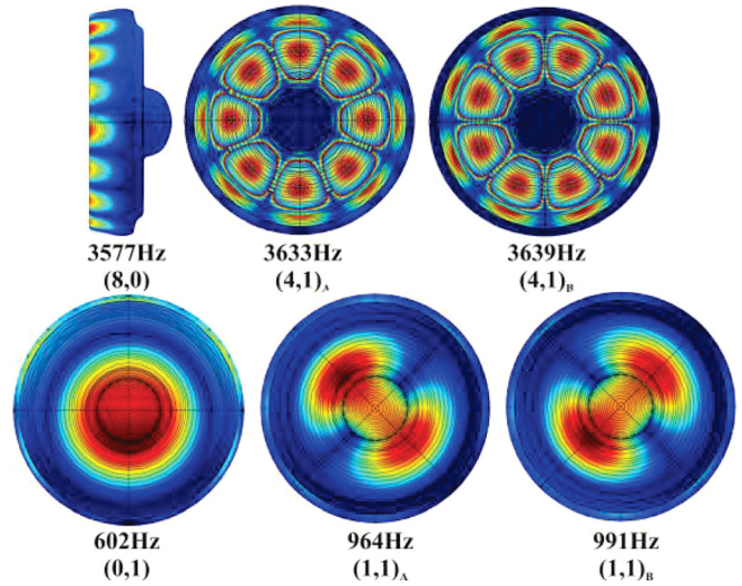
FIG. 3. (Color online) Selected modes predicted by the finite-element model.
