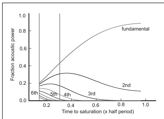
Figure 12. The normalized power in each harmonic component as a function of time to saturation of the lip opening, assuming the lip opening has the form shown in Figure 11. The curves are derived by calculating the power spectrum of equation (8). The vertical lines indicate the plausible range of the time to saturation in the experiments.
